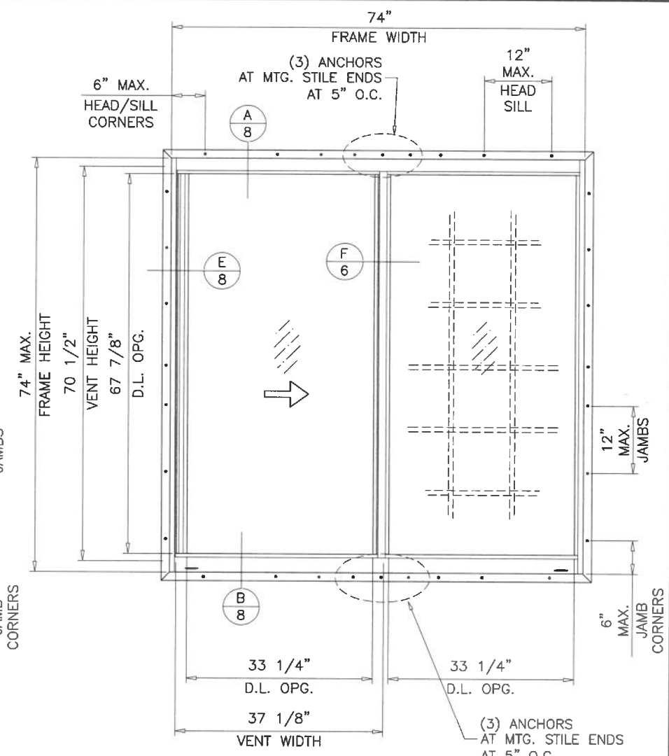
TYPICAL ELEVATION FLANGE FRAMES WITH FIN ADAPTER
